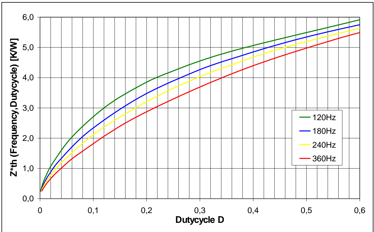
Figure 4: Thermal resistance for OSRAM OSTAR Projection module, pulsed operation of 2 chips
