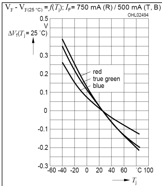
Figure 6: Relative Forward Voltage vs. Junction Temperature (e.g. OSRAM OSTAR Projection LE RTB-A2A)
