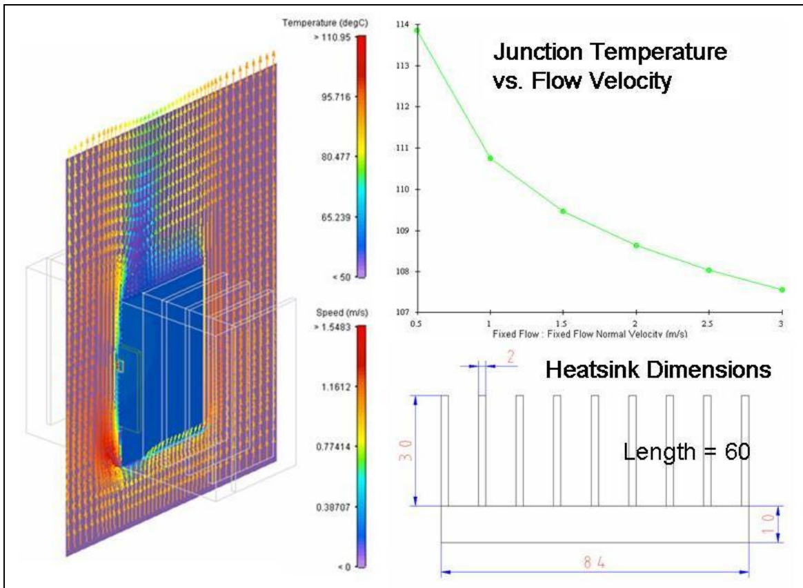
Figure 10: Simulation results of OSRAM OSTAR Projection with heat sink and fan
