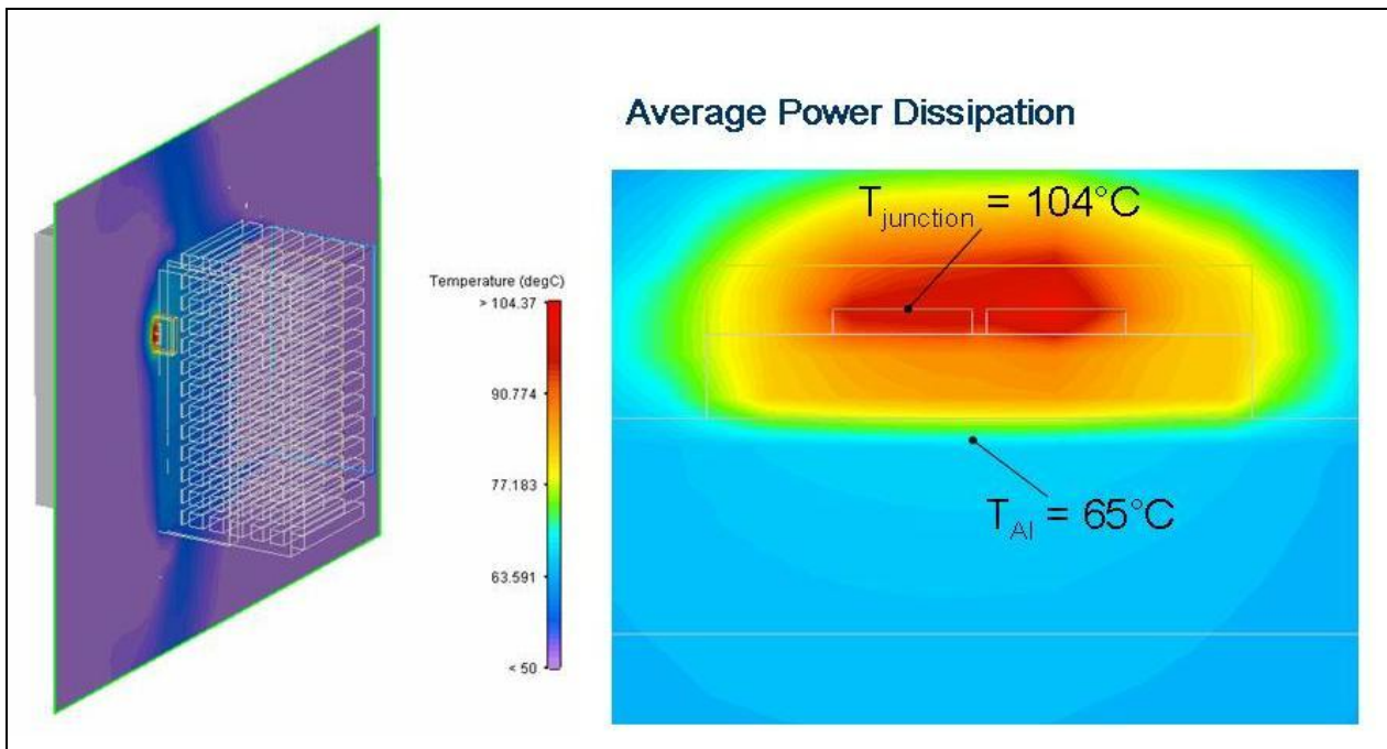
Figure 12: Simulation results of OSRAM OSTAR Projection in pulse operation, average temperature level
