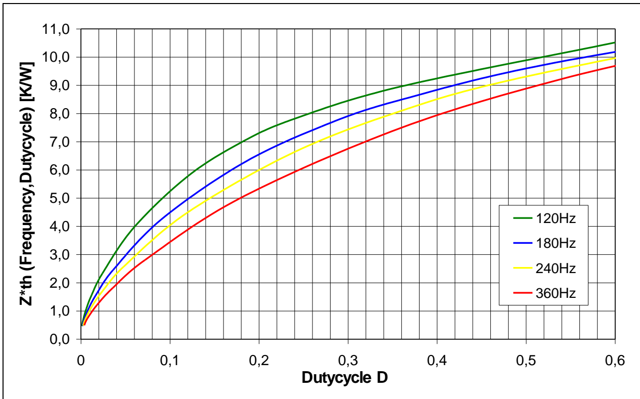
Figure 3: Thermal resistance for OSRAM OSTAR Projection module, pulsed operation of 1 chip
