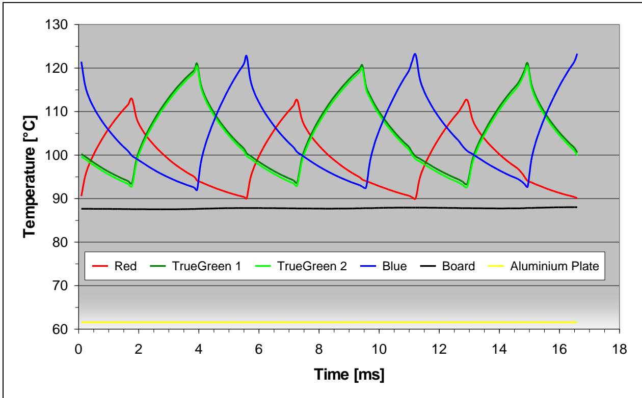
Figure 13: Simulation results of OSRAM OSTAR Projection in pulse operation, transient temperature curve
