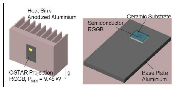
Figure 8: Construction of OSRAM OSTAR Projection with heat sink
