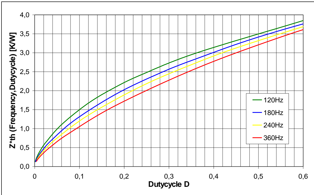
Figure 5: Thermal resistance for OSRAM OSTAR Projection module, pulsed operation of all 4 Chips
