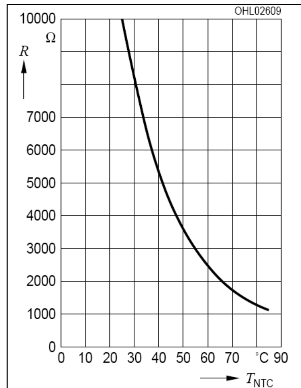
Figure 15: Typical thermistor graph (e.g. OSRAM OSTAR Projection LE B-A2A, NTC EPCOS 8502)
