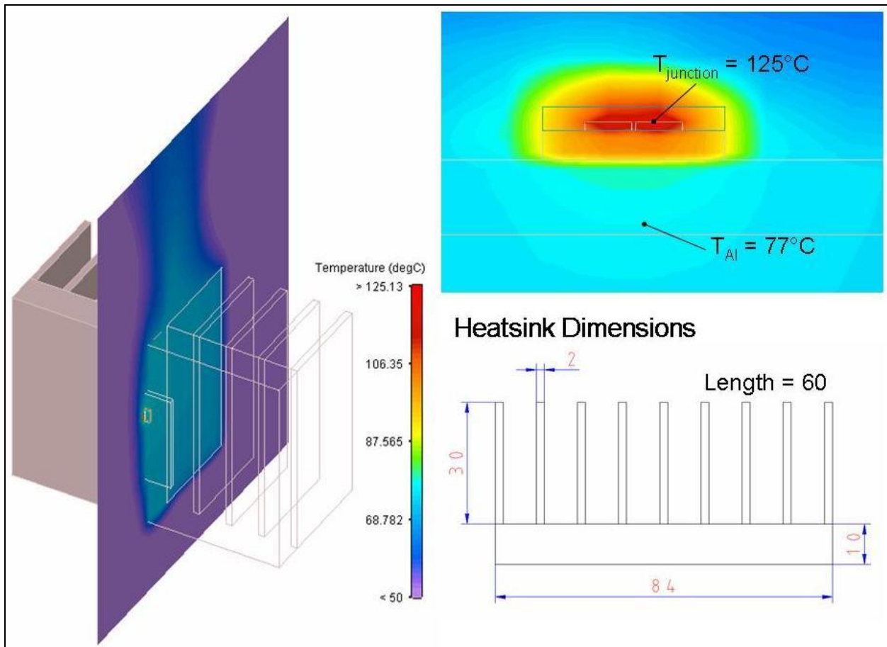
Figure 9: Simulation results for OSRAM OSTAR Projection with minimal heat sink
