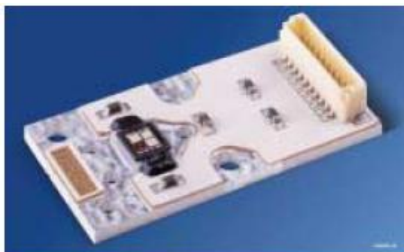
Figure 1: Construction of the OSRAM OSTAR Projection
