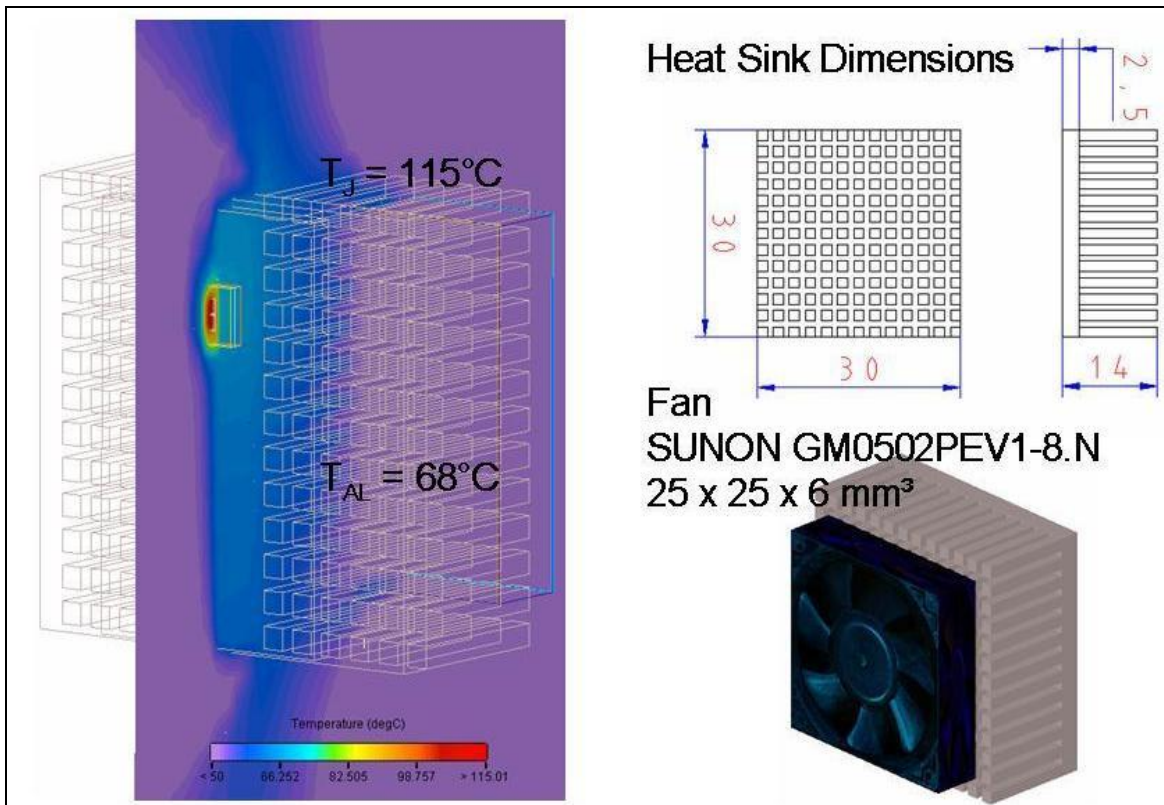
Figure 11: Simulation results of OSRAM OSTAR Projection with a minimized cooling element
