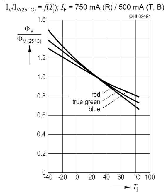
Figure 7: Relative Luminous Flux vs. Junction Temperature (e.g. OSRAM OSTAR Projection LE RTB-A2A)
