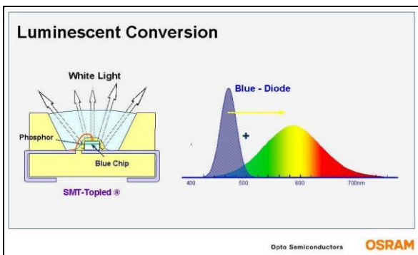
Figure 12: Principle for creating white light
